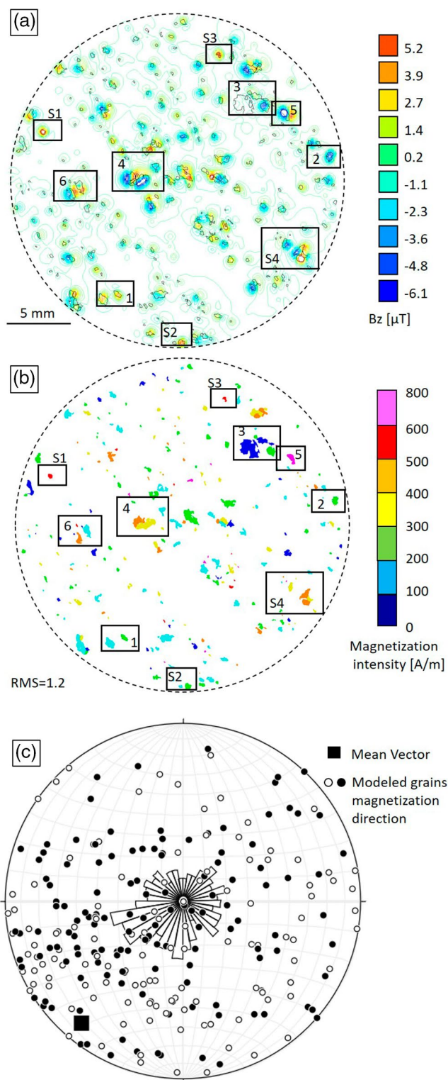
Figure 5. Data and inversion results prior to AF demagnetization. (a) Black boxes outline the area of the modeled grains. Overlaid are the contour lines of the magnetic data. (b) Bz full-scan inversion results with frustum bodies color coded by magnetization intensity in A/m. (c) Stereoplot of magnetization direction for each modeled body with 10° bin rose diagram in the middle. Closed circles are for positive inclinations and the square indicates the standard mean vector direction, 12° inclination and 219° declination, calculated from all modeled grains by adding up the direction cosines of all of the individual unit vectors. AF, alternating field.
