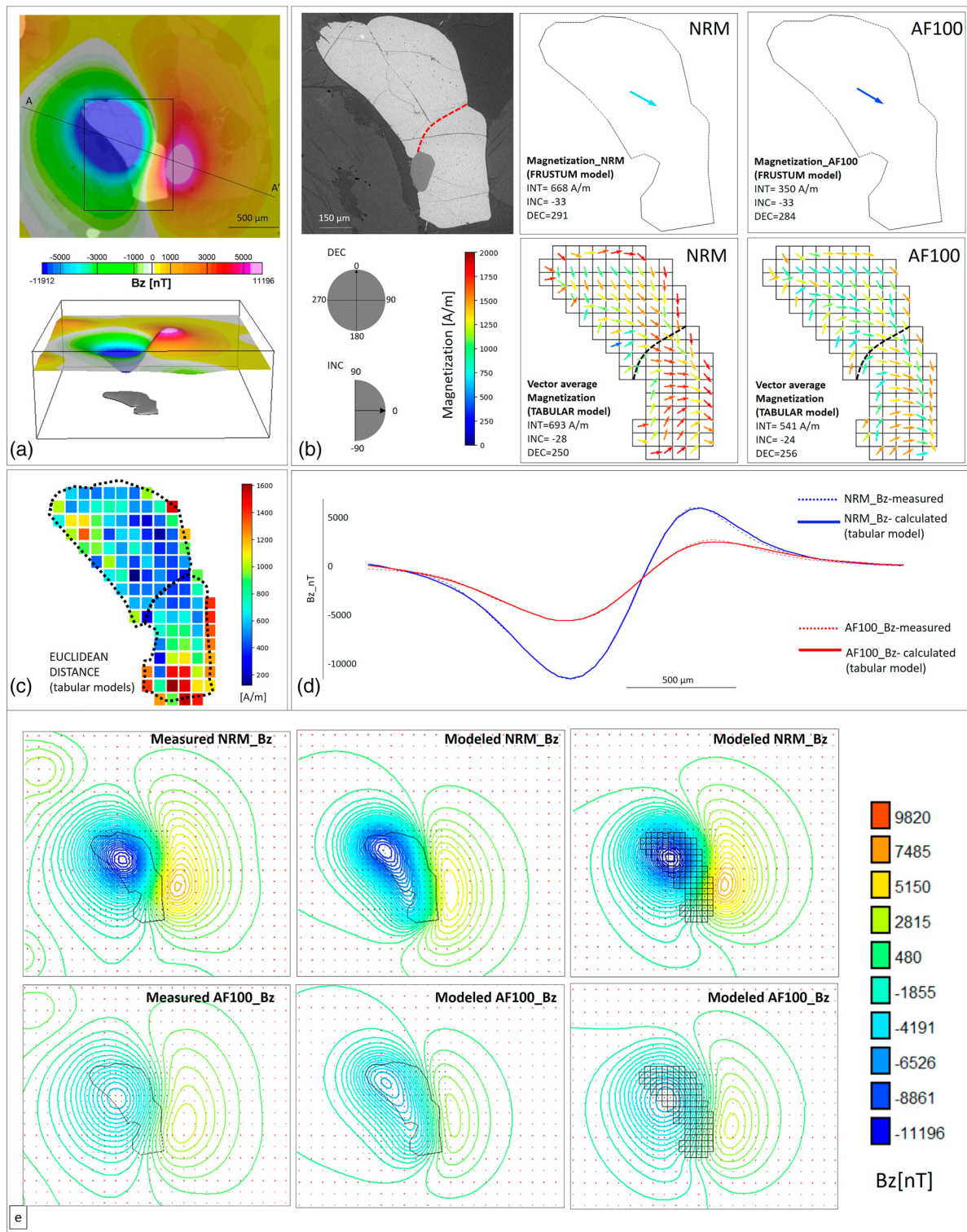
Figure 12. (a) Map and 3D views of the magnetic anomaly measured over the grains in area 5, Figure 4. (b) SEM image, and frustum and tabular models of the grain/grains obtained by inverting NRM_Bz and AF100_Bz scan data. The red dashed line on the SEM image indicates a grain boundary, traced based on the observation of a different orientation of the exsolution lamellae in two areas. Arrows on top of tabular bodies are color coded by magnetization intensity and oriented according to inclination angle. (c) Comparison of NRM and AF100 tabular-body models with each body colored according to the calculated Euclidian distance. (d) Profile AA' (see Bz map in a for profile location) with modeled (tabular-body models) and calculated Bz for NRM and AF. (e) Contour lines and profile with calculated and measured Bz for NRM and AF both for frustum and tabular bodies. Red points on contour maps are data points where the Bz is calculated. SEM, scanning electron microscope; NRM, natural remanent magnetization; AF, alternating field.
