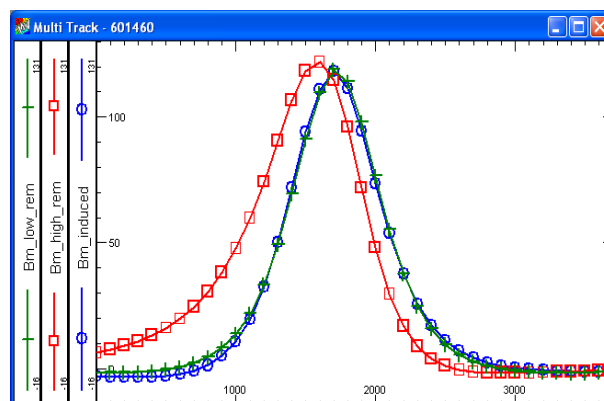
Figure 1. Example east west profiles over a vertical magnetic pipe (D) showing the results for induced magnetization (blue circles), weak remanence (green +) and strong remanence (red square).
